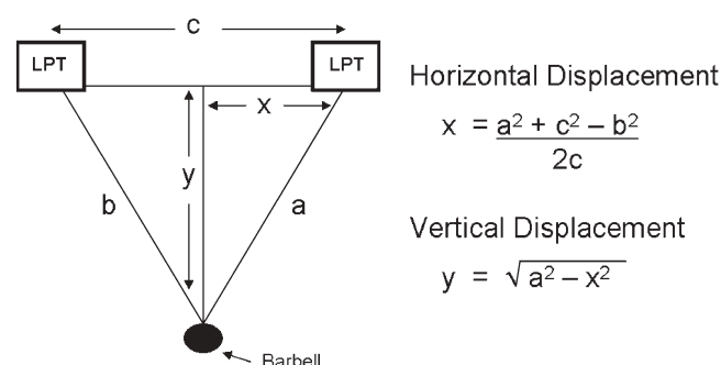
FIGURE 1 —Two LPT configuration used for the calculation of vertical and horizontal displacement; a and b , voltage output from LPT converted to displacement values through calibration to known distances; c , constant distance between LPT; x , horizontal displacement; y , vertical displacement.
