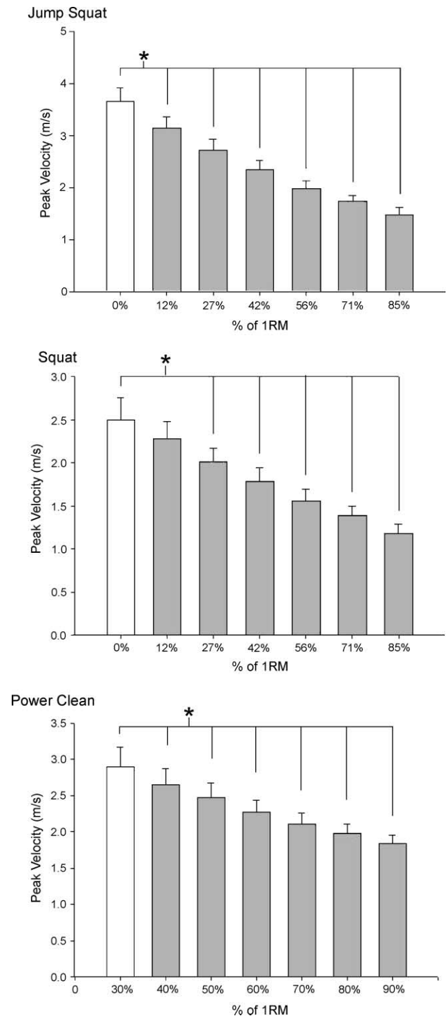
FIGURE 7 —Peak velocity across the loading spectrum in the JS, S, and PC. * Significant ( P \leq 0.05 ) difference between load that maximized peak velocity (designated by open bar) and the peak force at other loads within the same lift.
