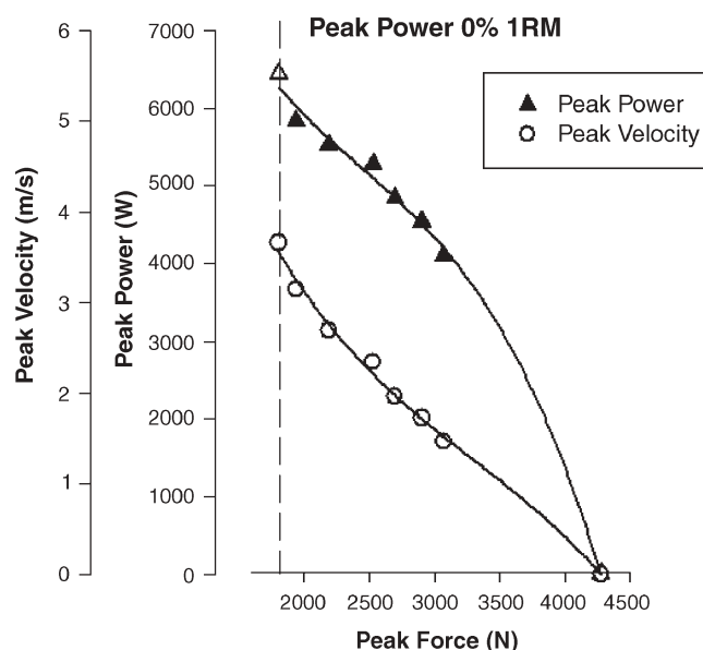
FIGURE 2 —Force-velocity and force-power plots for the JS. Absolute peak power is designated by solid triangles ; peak velocity is denoted by open circles . Optimal load is identified by an open triangle .
